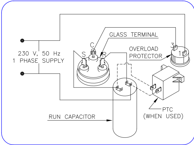
PERMANENT SPLIT CAPACITOR (PSC)
