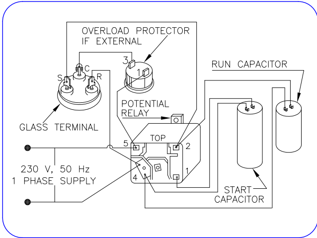
CAPACITOR START CAPACITOR RUN (CSCR) WITH POTENTIAL RELAY
