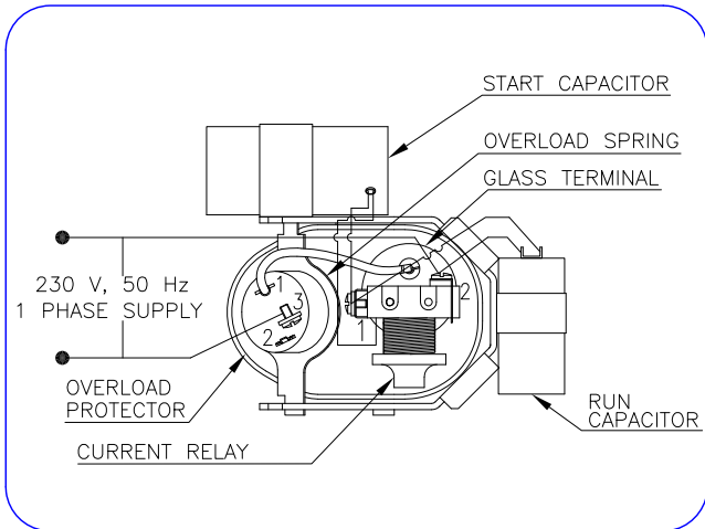
CAPACITOR START CAPACITOR RUN (CSCR) WITH PLUG-IN CURRENT RELAY
