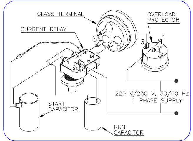
CAPACITOR START CAPACITOR RUN (CSCR) WITH NTC RELAY
