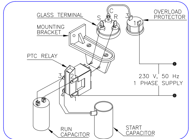
CAPACITOR START CAPACITOR RUN (CSCR) WITH PTC RELAY (8EA19D7)
