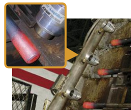
Model 6042 2" (51mm) Adjustable Air Amplifiers with swivel fittings cool inductively heated axles prior to installing the hubs.
