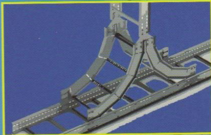
TWO SIDE VERTICLE BEND
