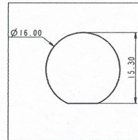
PANEL CUTOUT FOR PLUG MOUNTING
