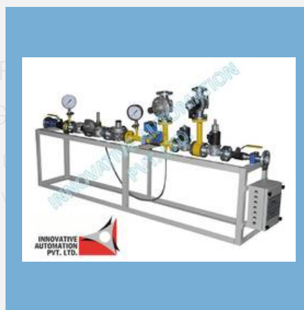
Straight Design Prepiped Gas Trains
