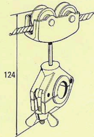
JUMBO TYPE WITH BUSH - 25 MM Ø in POLYPROPYLENE
