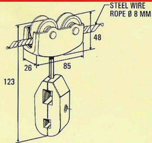
ROUND TYPE in NYLON in POLYPROPYLENE
