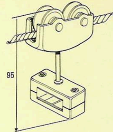
FLAT TYPE in NYLON in POLYPROPYLENE
