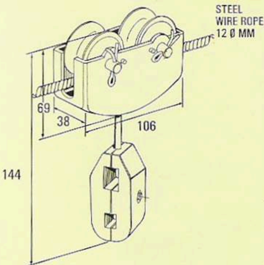
ROUND TYPE in NYLON in POLYPROPYLENE
