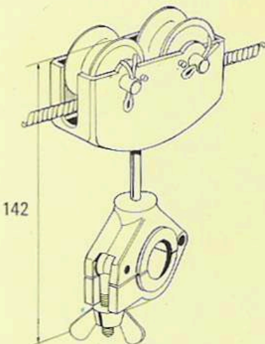
JUMBO TYPE WITH BUSH 25 MM Ø in POLYPROPYLENE
