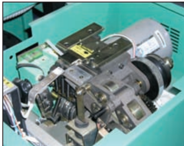
Electronic tension adjustment for variable tension
