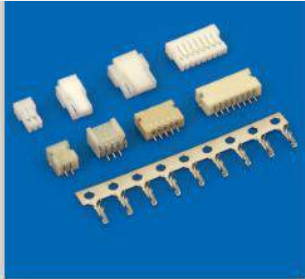
1mm Pitch ST-A1002 (NH1.0)
