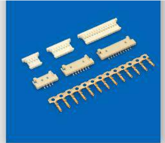
1.25mm Pitch ST-A1254
