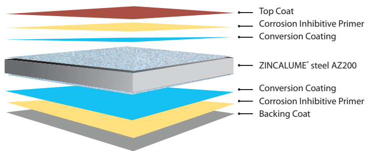
Cross Section View of COLORBOND® Ultra steel
